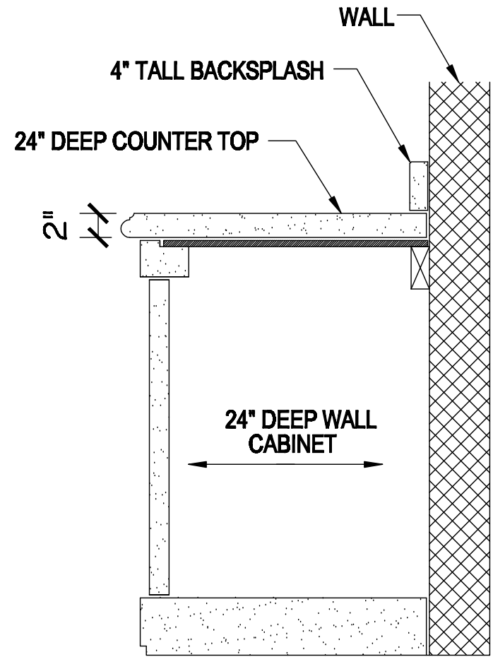
24" DEEP WALL CABINET WITH 24" DEEP COUNTER TOP
